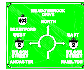
TYPICAL GUIDE SIGN EAST & WEST APPROACHES INSTALL 150m FROM ROUNDABOUT
