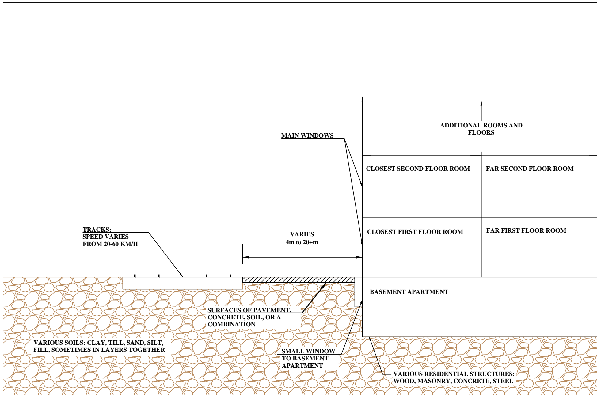
FIGURE 2 SOURCE-RECEIVER CONFIGURATION
