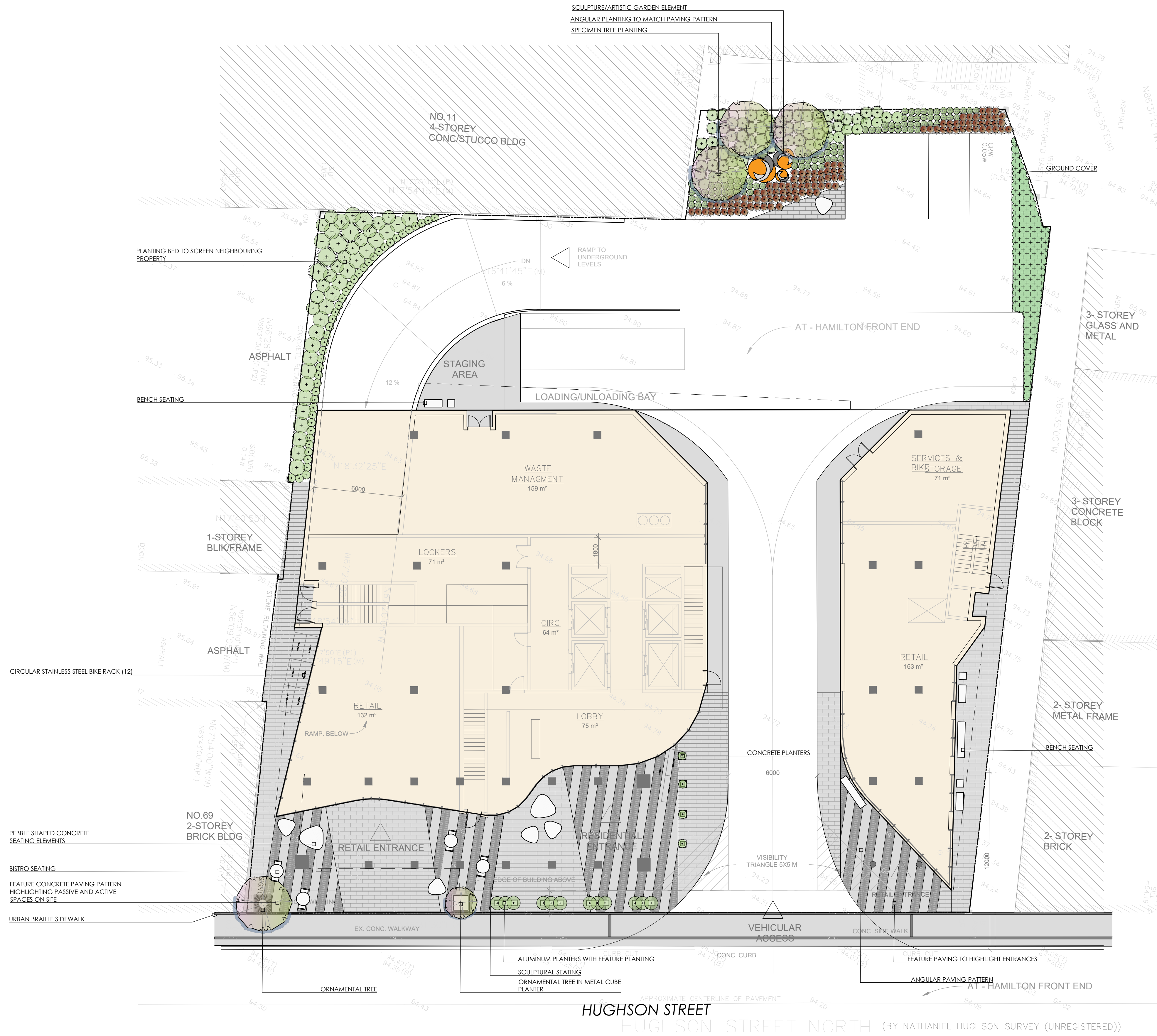
LINEAR PAVING AND ANGULAR SEATING ELEMENTS
