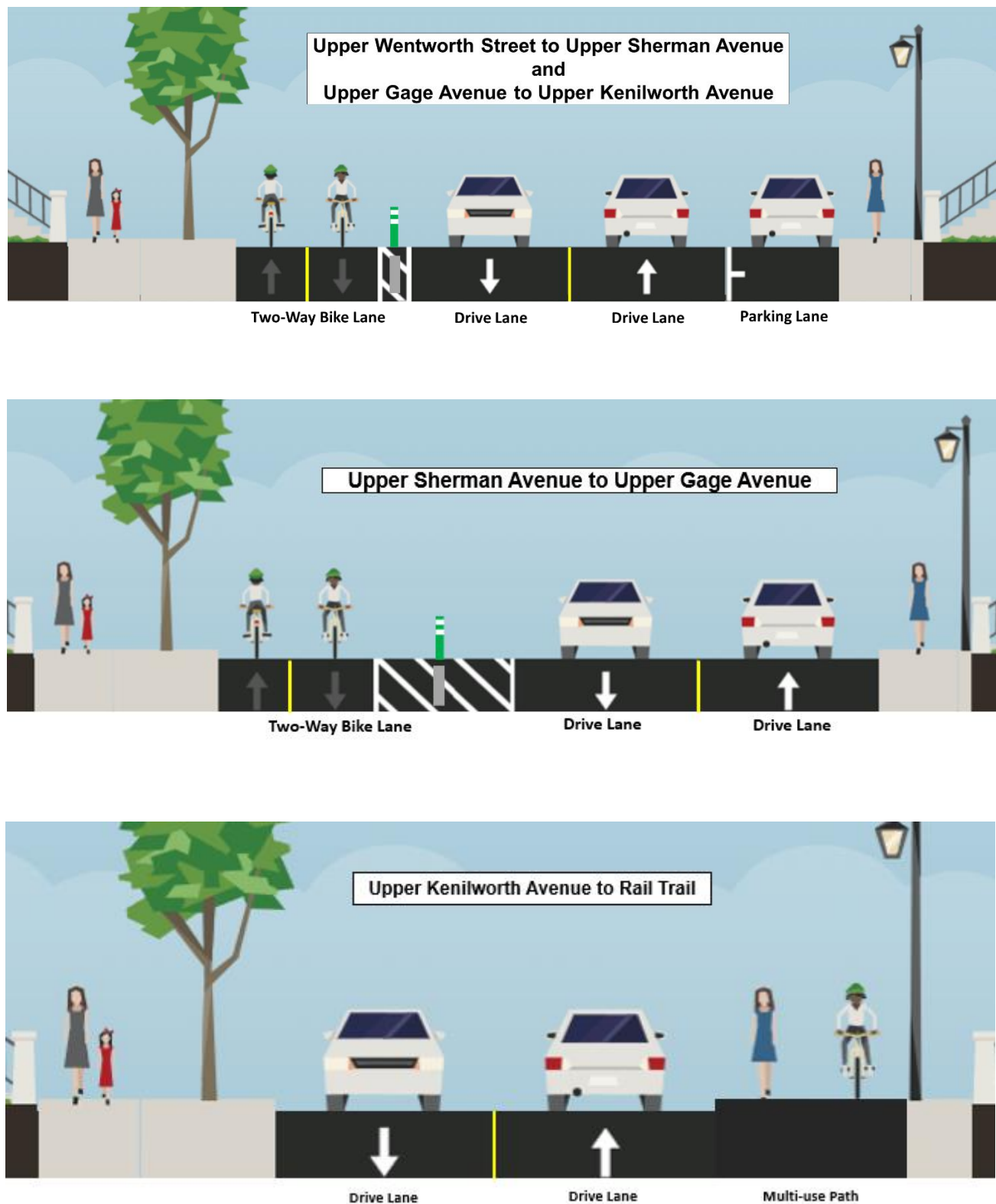
Figure 2 - Limeridge Road Proposed Lane Arrangement
