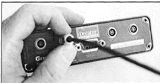
Figure 2.2b Align the red dot on the connector with the red dot on the computer receptacle.
