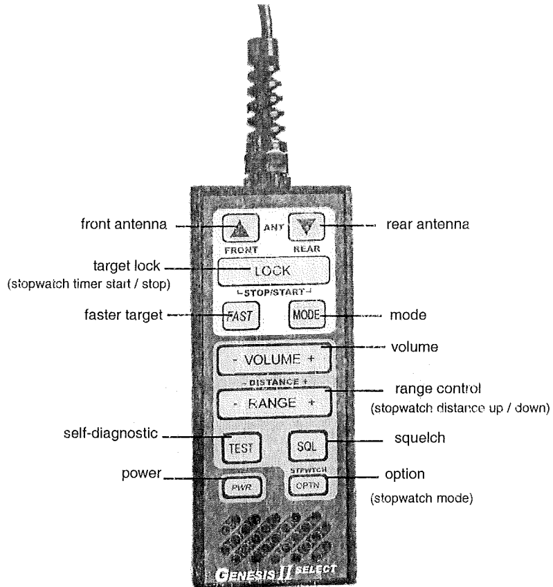
Figure 6 The hand-held remote control unit.
