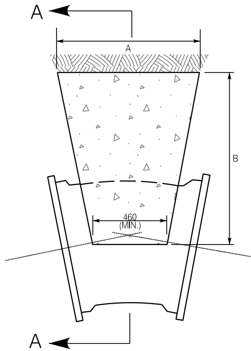
PLAN VIEW
