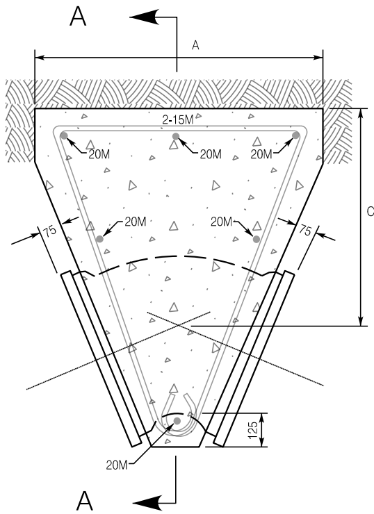
PLAN VIEW
