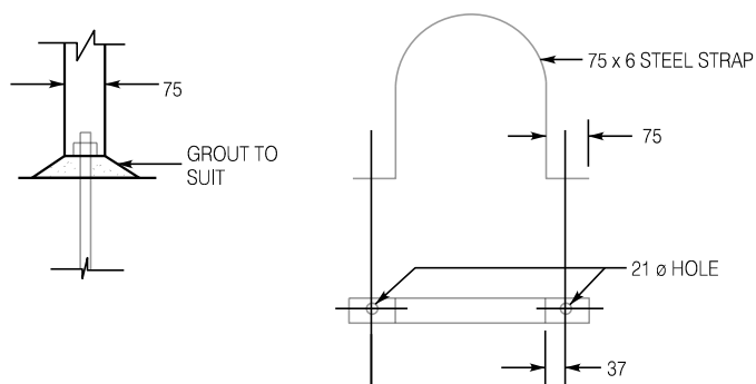
STEEL STRAPPING DETAILS
