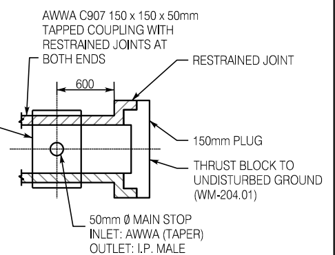
PVC INSTALLATION
