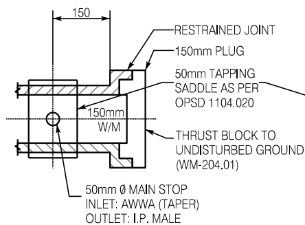
DUCTILE IRON INSTALLATION
