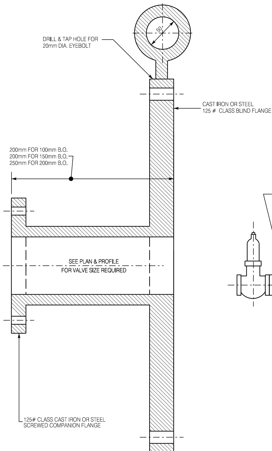
TYPICAL FLANGE SECTION
