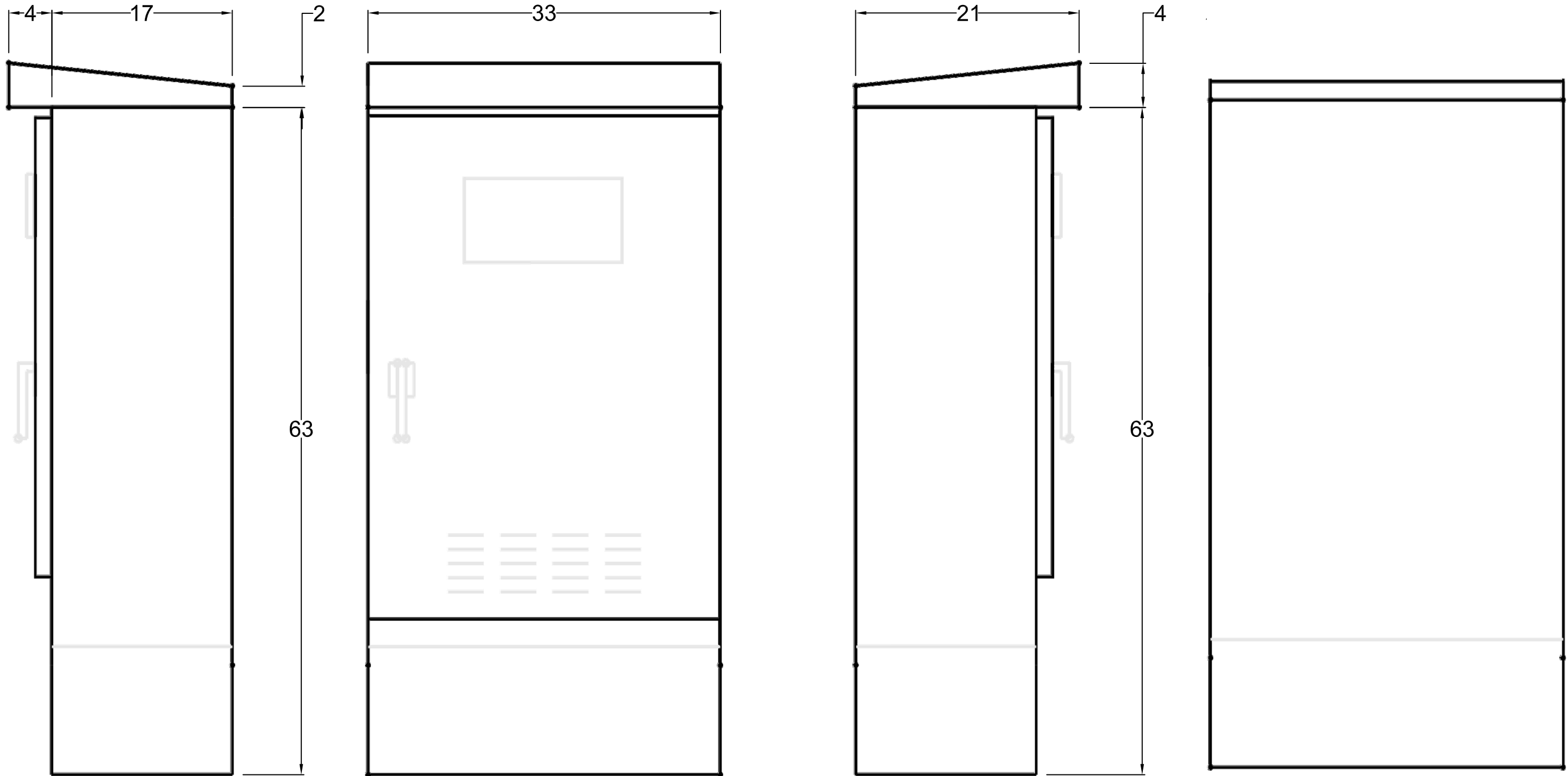
FRONT VIEW
